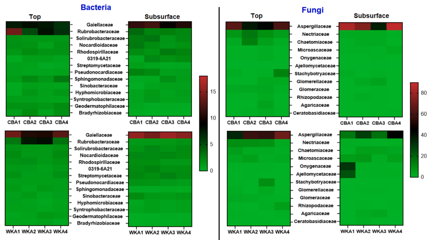
Fig. 7. The most dominant bacterial and fungal families for CBAi and WKAi (i = 1, 2, 3 and 4).
