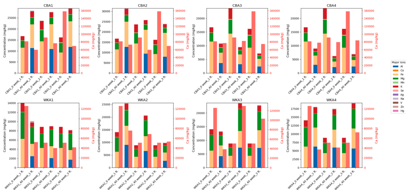
Fig. 3. The major metal and metalloid composition at 1 ft., 2 ft., and 3 ft. of CBAi and WKAi ( i = 1, 2, 3 and 4) fluctuates over time. The ion concentration of the 0th week and 40th week is shown for all the depths, and the compounds are color-coded.
