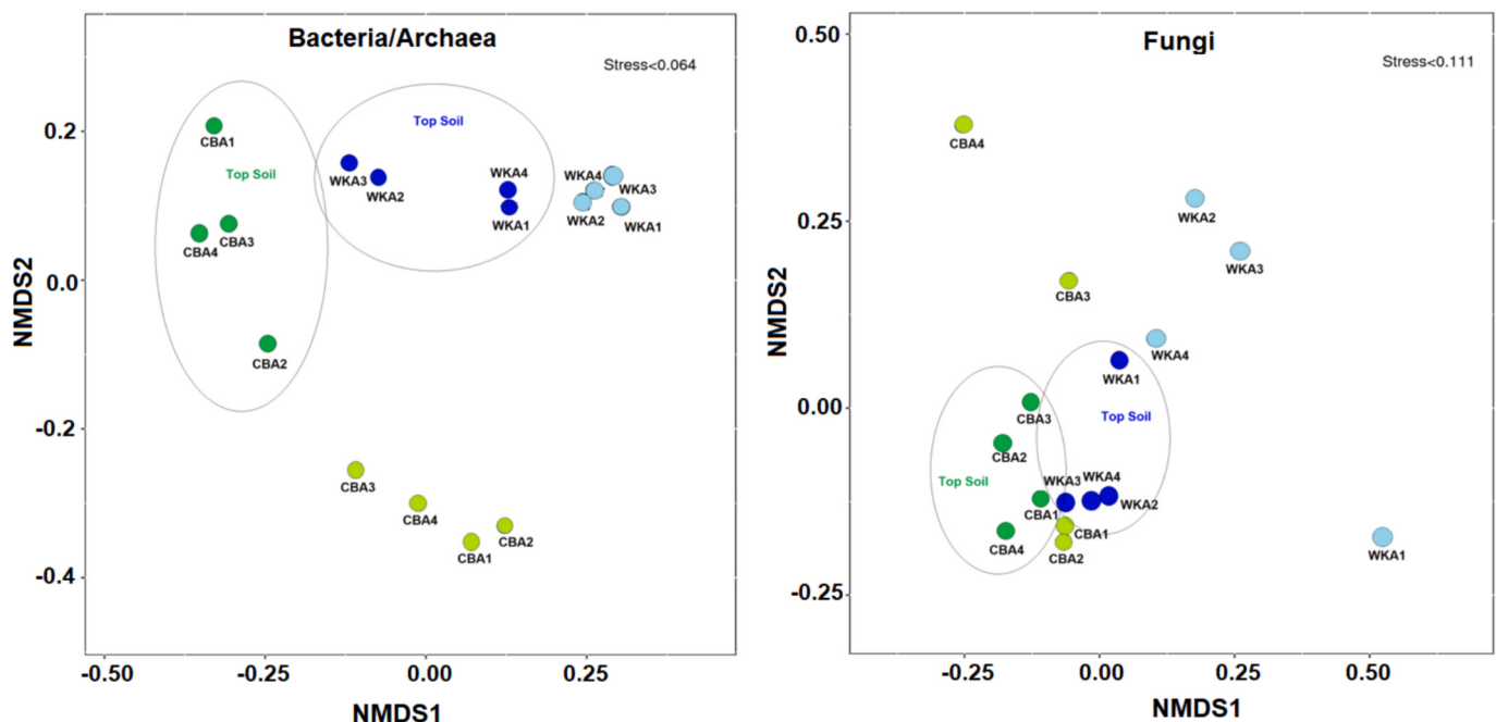
Fig. 8. The NMDS figures to show the similarity of the bacterial/archaeal and fungal community for CBAi and WKAi ( i = 1, 2, 3 and 4). (green: top CB soil; light green: subsurface CB soil; blue: top WK soil; light blue: subsurface WK soil).
